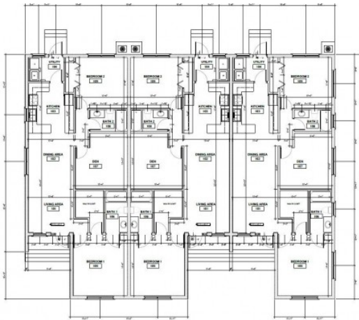
1 GROUND FLOOR PLAN Scale: 1/8" = 1'-0"
