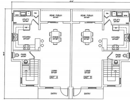
1 LEVEL 1 FLOOR PLAN 1/4" = 1'-0" LEVEL 1 = 141 SF LEVEL E = 141 SF TOTAL = 282 SF
